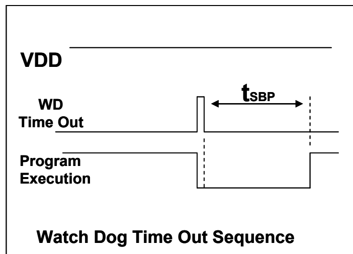
Fig.18: Sequence of Watch Dog Time Out
