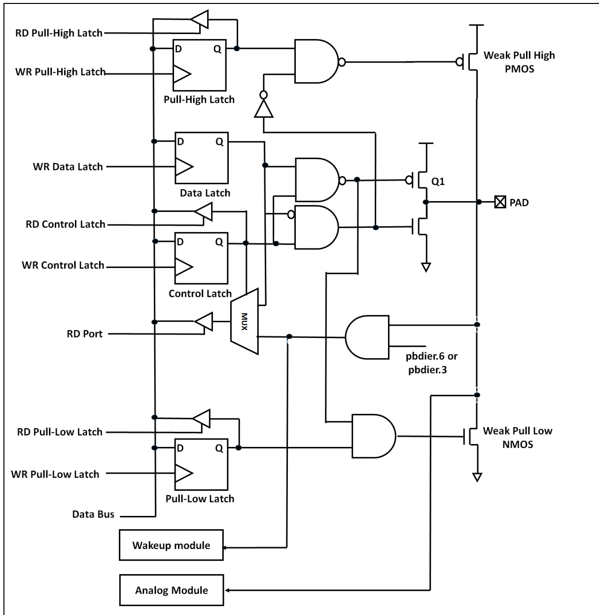
Fig.20: Hardware diagram of IO buffer
