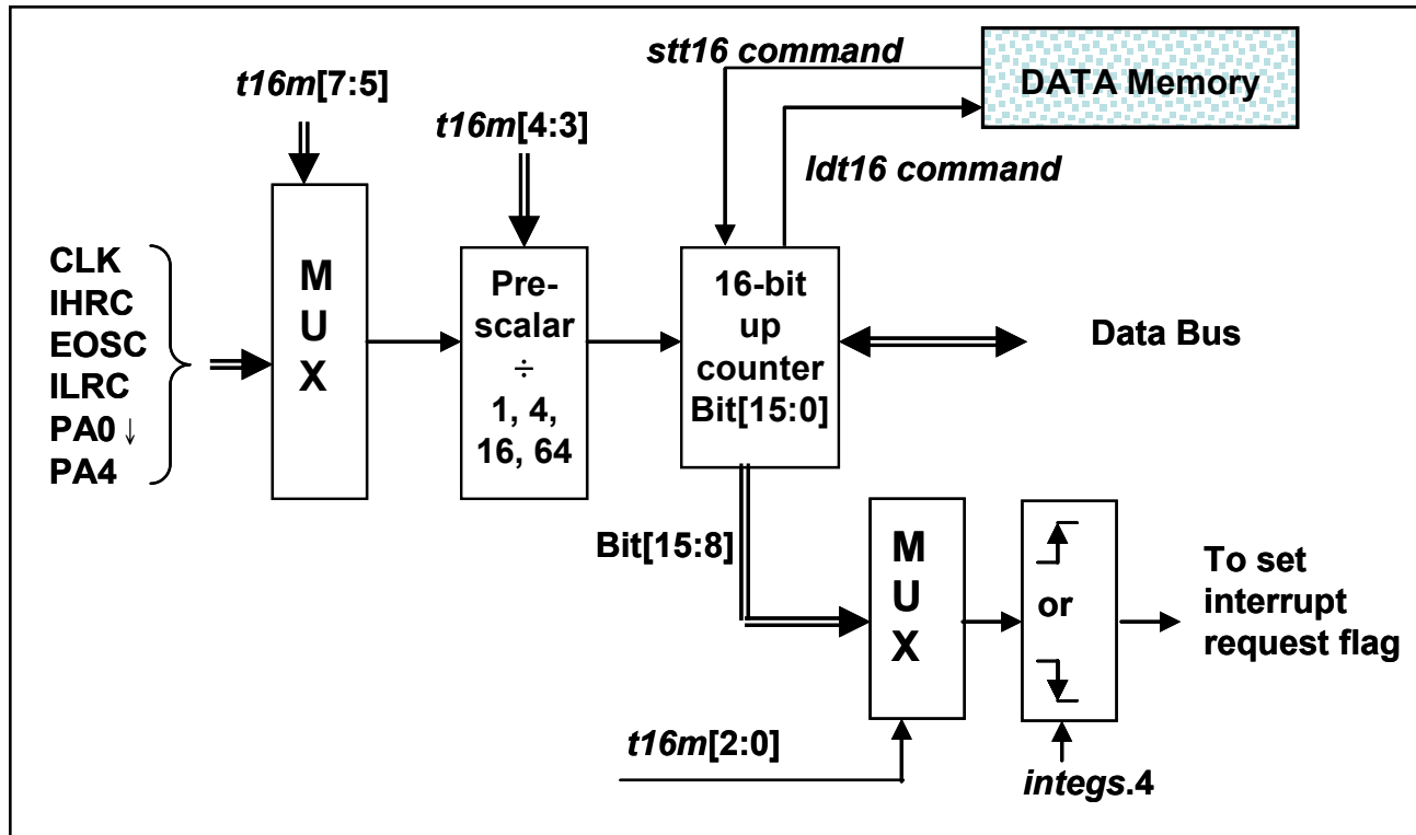
Fig.10: Hardware diagram of Timer16
