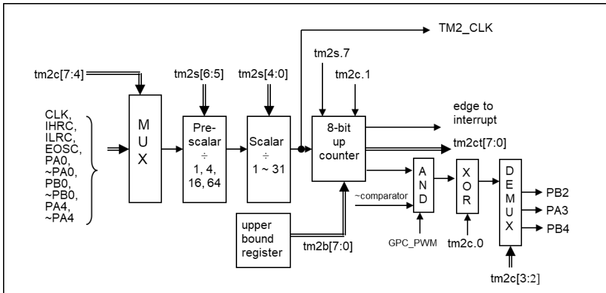
Fig.11: Timer2 hardware diagram
