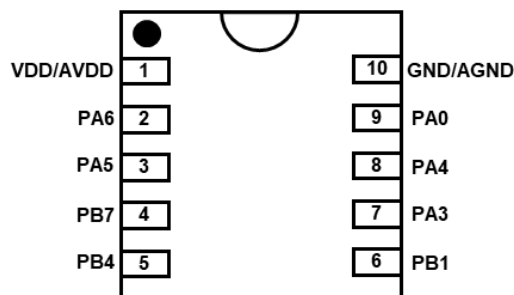
PFS132-4N10: DFN3*3-10pin (0.5pitch)
