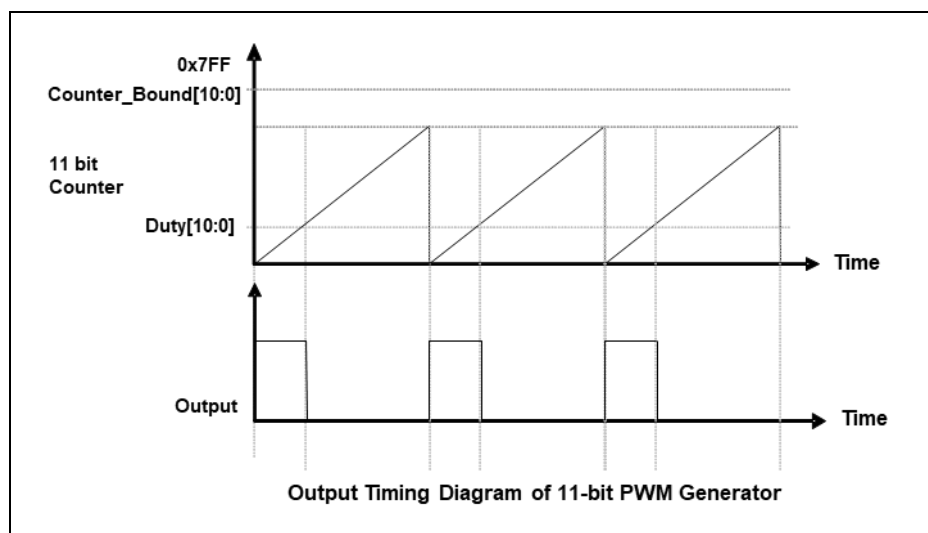
Fig.16: Output Timing Diagram of 11-bit PWM Generator
