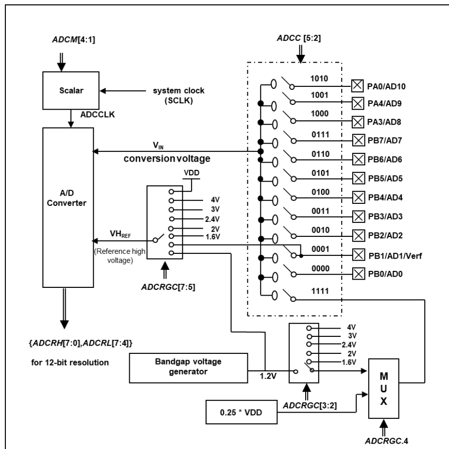
Fig.21: ADC Block Diagram
