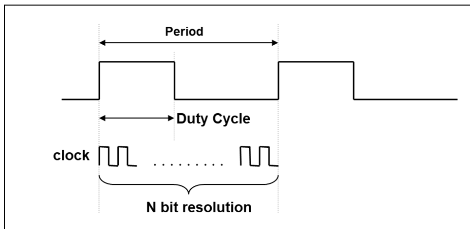
Fig.14: PWM Output Waveform
