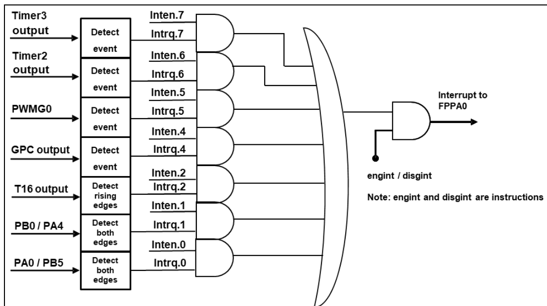
Fig.19: Hardware diagram of interrupt controller
