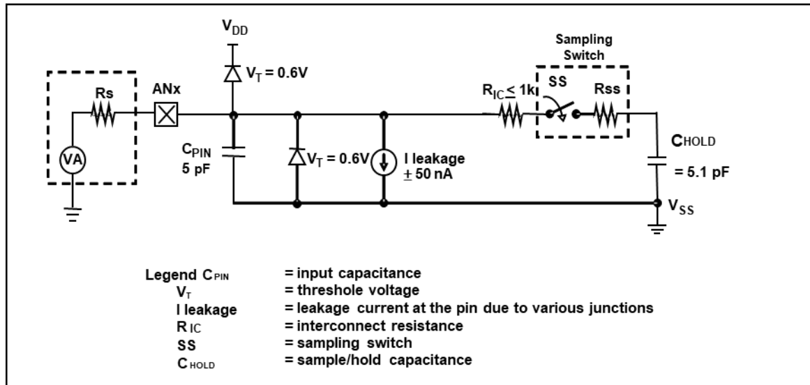
Fig.22: Analog Input Model
