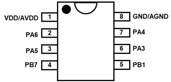
PFS132-S08: SOP8 (150mil)
