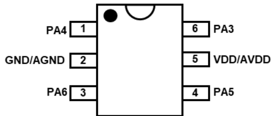
PFS132-U06: SOT23-6 (60mil)
