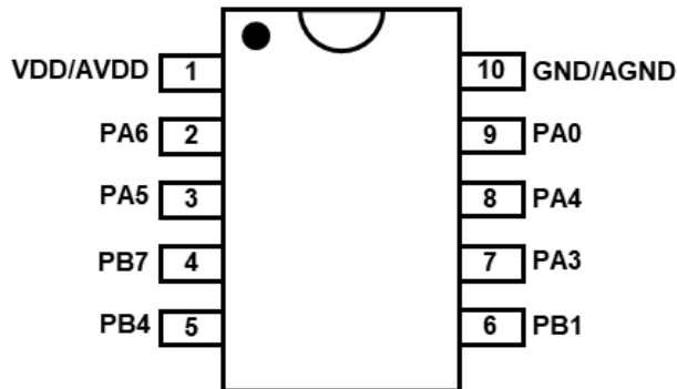
PFS132-M10: MSOP10 (118mil)
