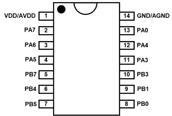
PFS132-S14: SOP14 (150mil)
