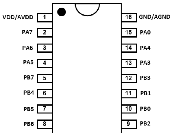
PFS132-S16A: SOP16 (150mil)
