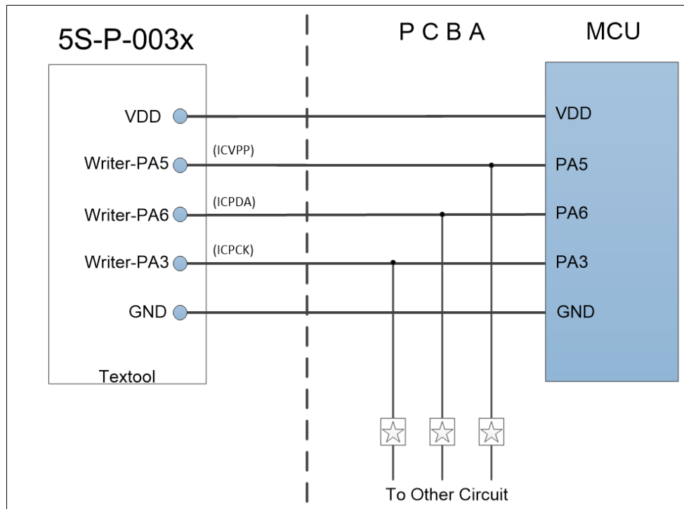
Fig. 24: Schematic Diagram of On-Board Wiring
