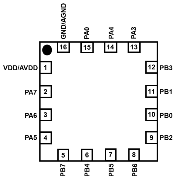
PFS132-1J16A: QFN3*3-16pin (0.5pitch)
